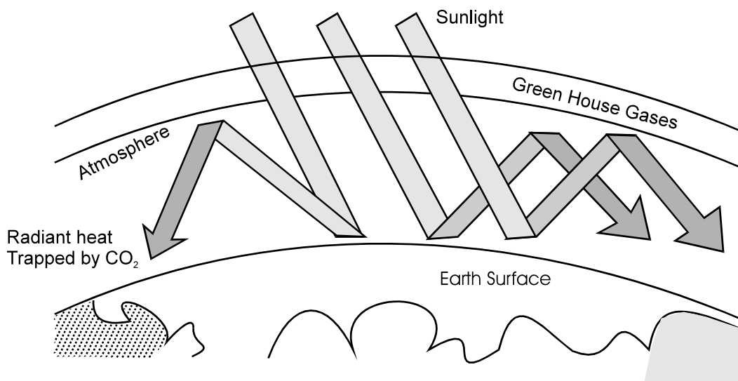
Fig. The green house effect of \text{CO}_2
