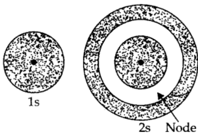
Fig. 2.9 Shapes of 1s and 2s orbitals.
