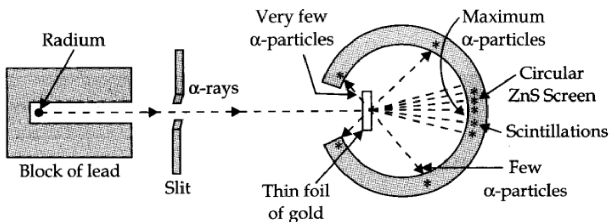
Fig. 2.3 Rutherford's scattering experiment.
