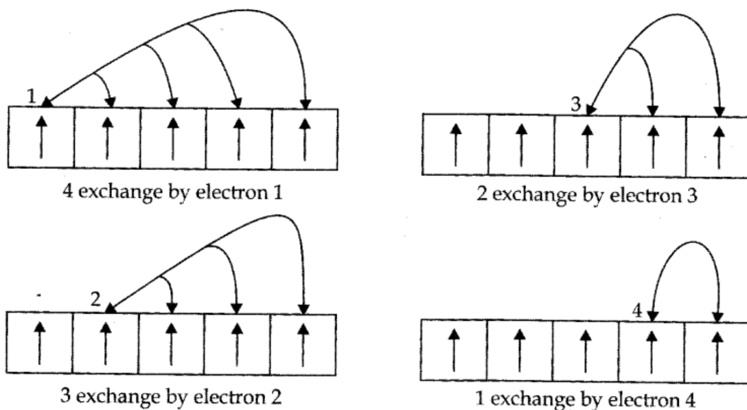
Fig. 2.12 Possible exchange for a d^5 configuration.
