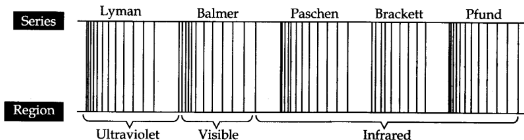
Fig. 2.8 Atomic spectrum of hydrogen.
