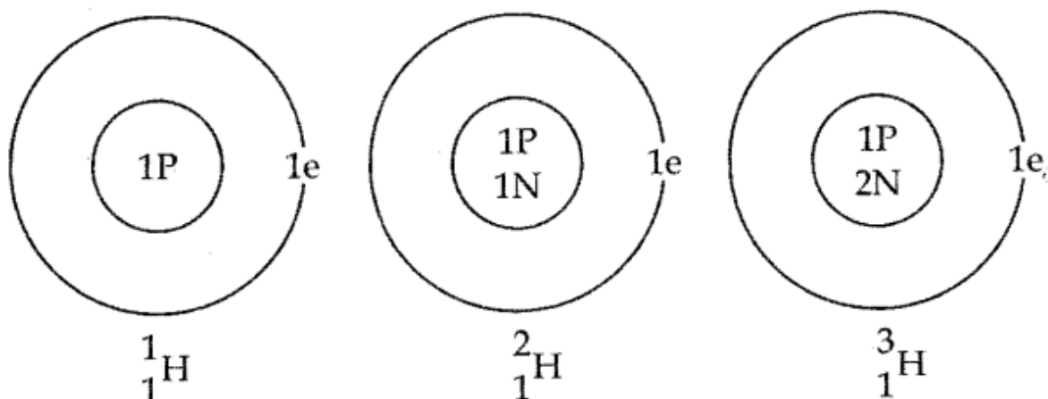
Fig. 2.4. The three isotopes of hydrogen.
