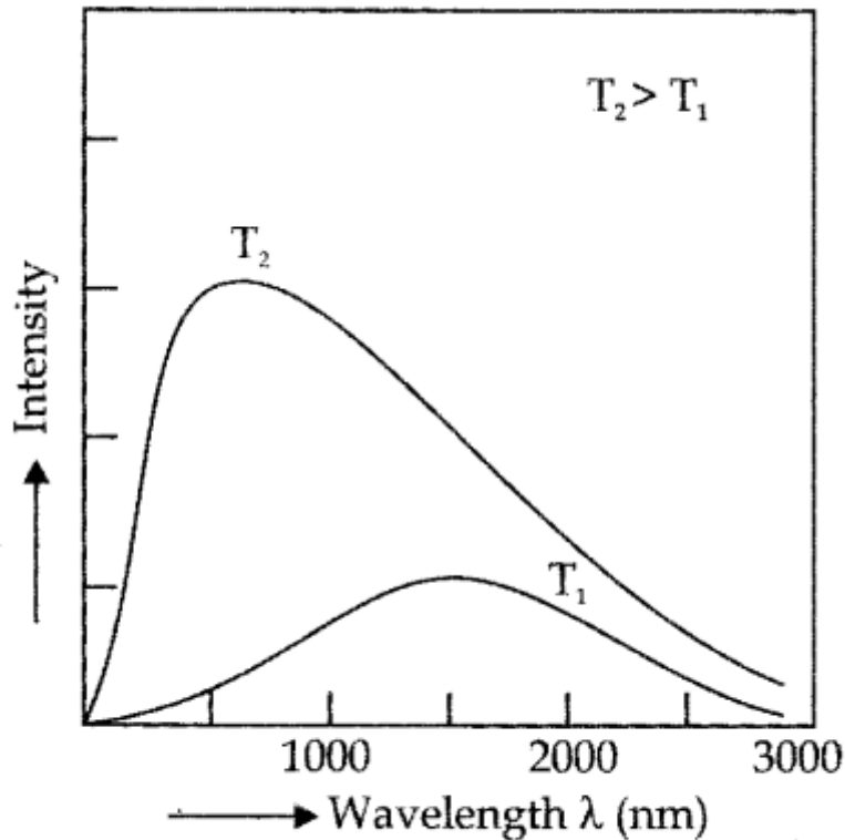
Fig. 2:6 Wavelength-intensity relationship.
